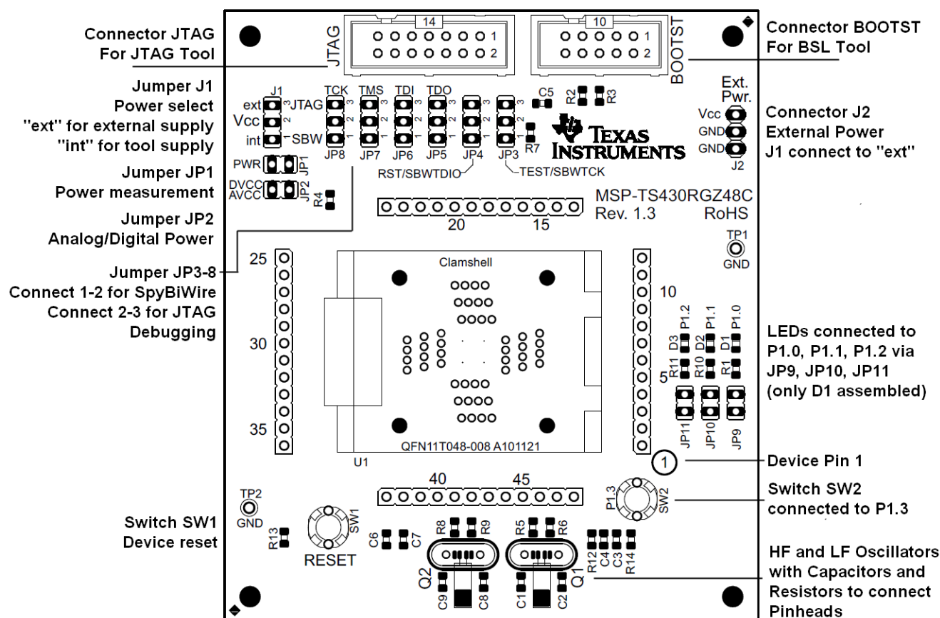
Figure B-30. MSP-TS430RGZ48C Target Socket Module, PCB
