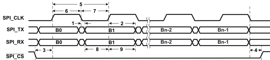
Figure 6-34. SPI Mode 0 Transfer (CKP n = 0, CKPH n = 0)
