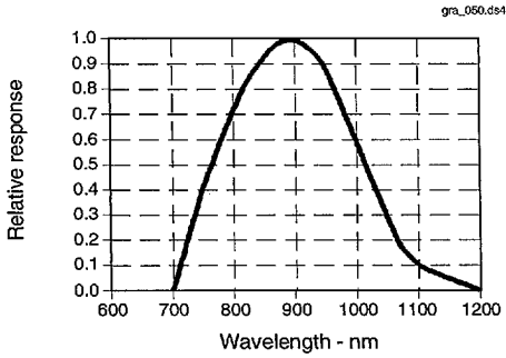
Fig. 5 Spectral Responsivity
