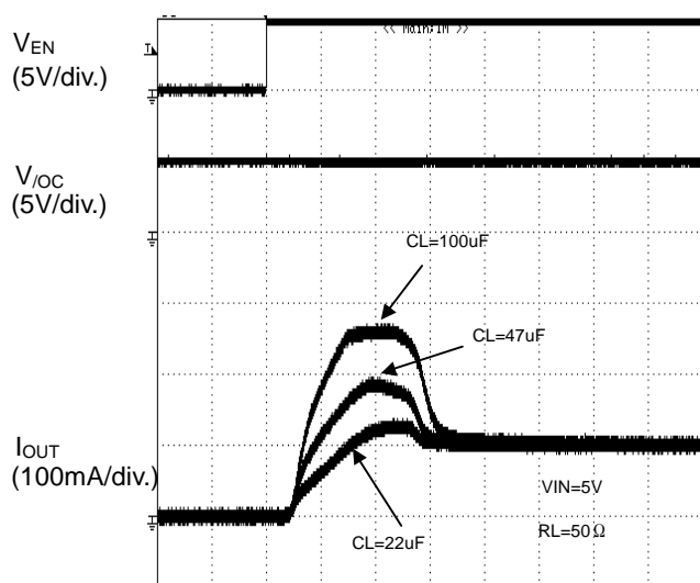
Figure 56. Inrush Current Response
