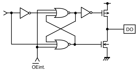
Figure 36. Output Circuit (DO)
