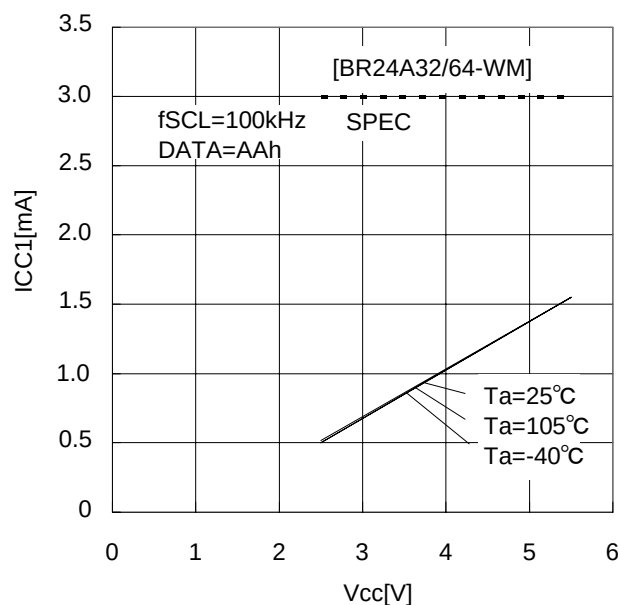
Figure 11. Current consumption at WRITE operation ICC1 ( f_{SCL}=100\text{kHz} )
