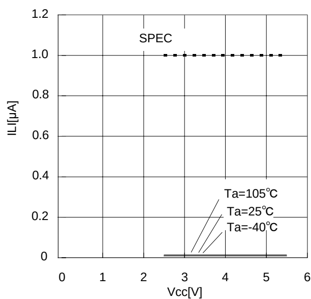
Figure 5. Input leak current I_{LI} (SCL, WP)
