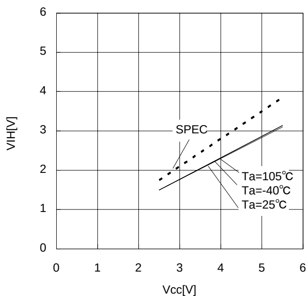
Figure 2. H input voltage V_{IH1,2} (SCL, SDA, WP)
