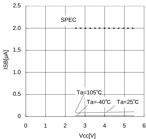
Figure 13. Standby current ISB
