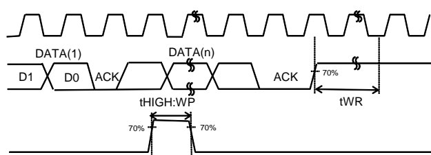
Figure 2-(e). WP Timing at Write Cancel
