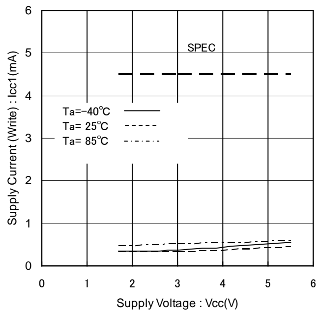
Figure 11. Supply Current (Write) vs Supply Voltage ( f_{SCL}=1\text{MHz} BR24G1M-3A)
