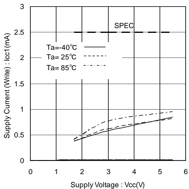
Figure 10. Supply Current (Write) vs Supply Voltage ( f_{SCL}=1\text{MHz} BR24G128/256-3A)
