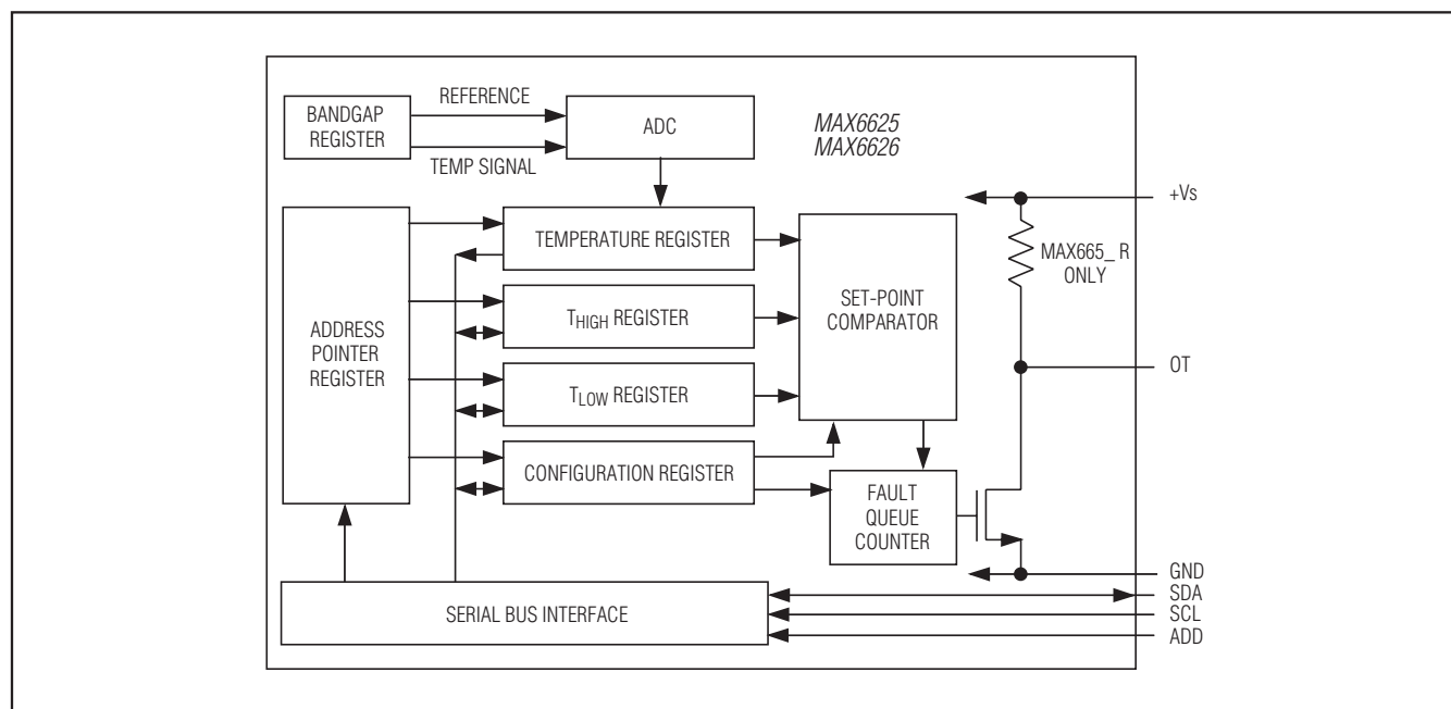
Figure 2. Functional Diagram
