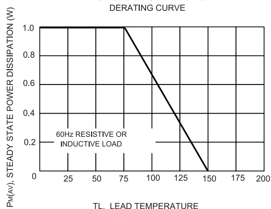
FIG.4-STEADY STATE POWER DERATING CURVE
