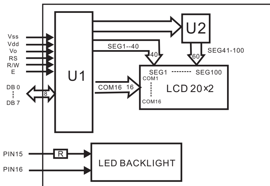
Block Diagram
