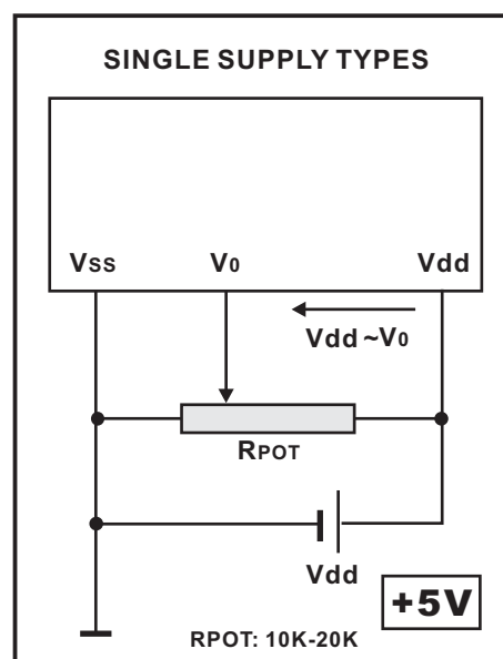
Power Supply Diagram
