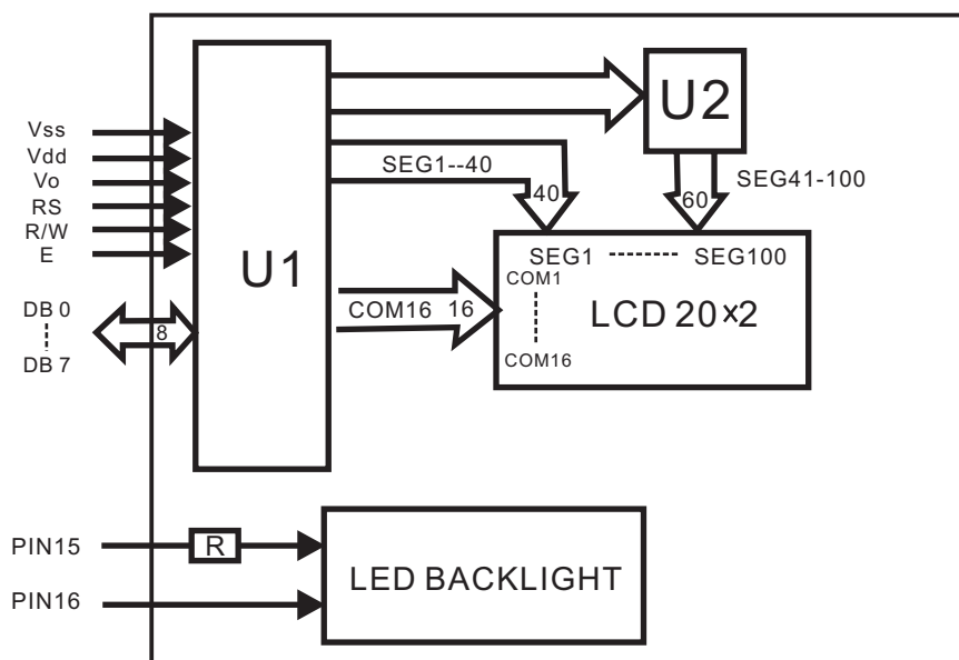
Block Diagram
