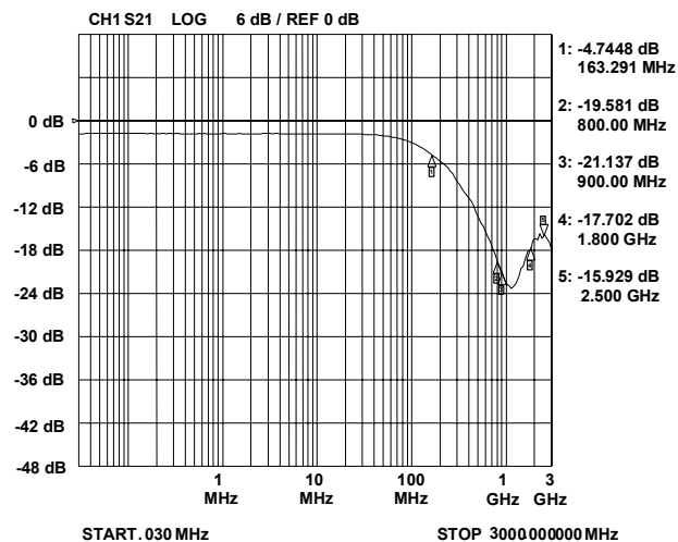
Typical Insertion Loss S21
