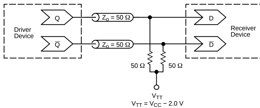
Figure 16. Typical Termination for Output Driver and Device Evaluation (See Application Note AND8020/D – Termination of ECL Logic Devices.)
