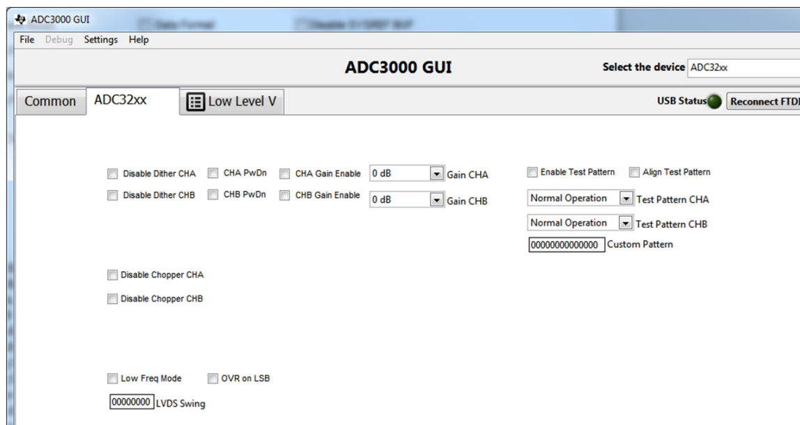
Figure 9. ADC32xx Tab
