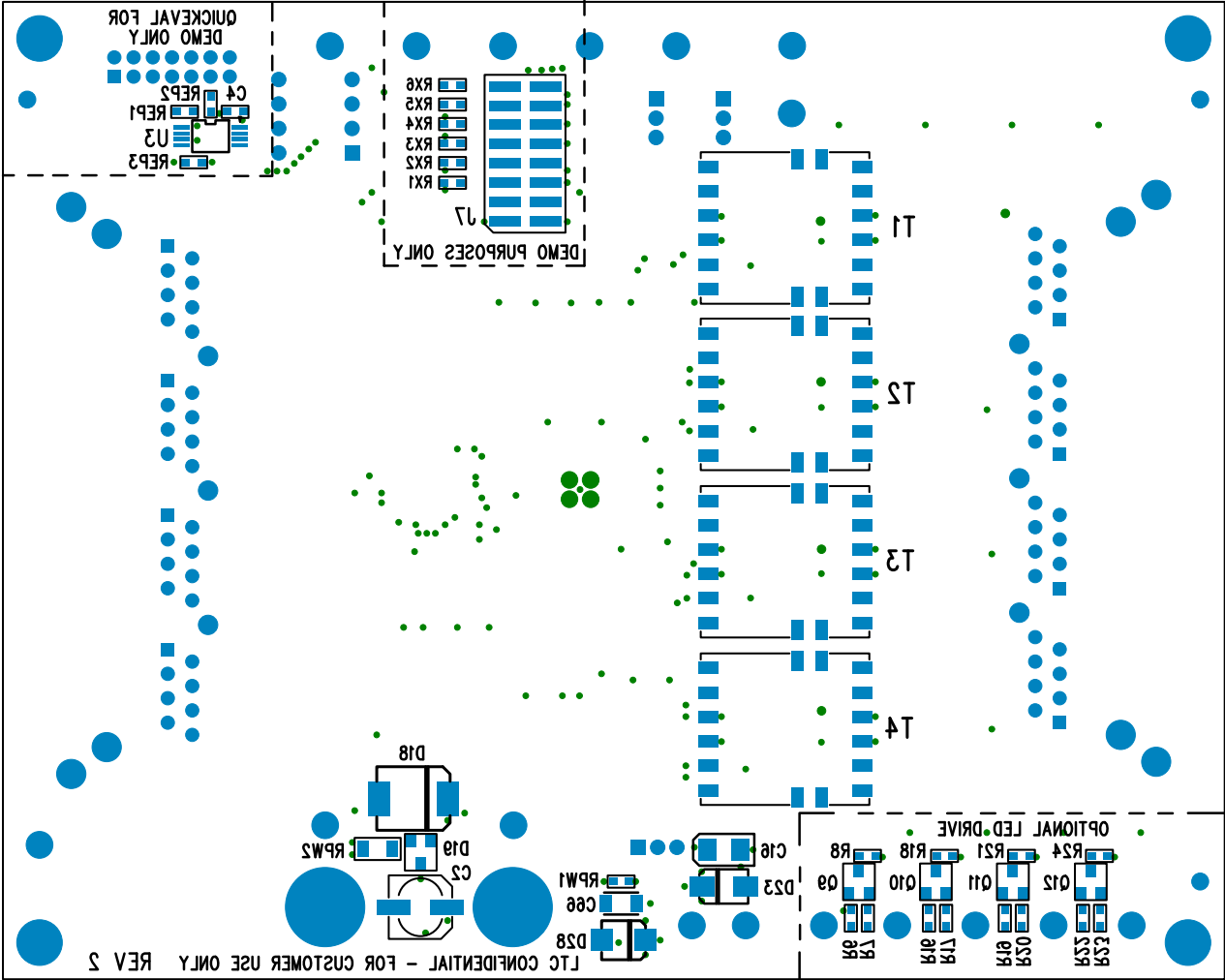
Bottom Assembly
