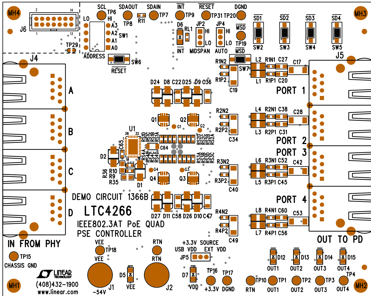
Top Assembly
