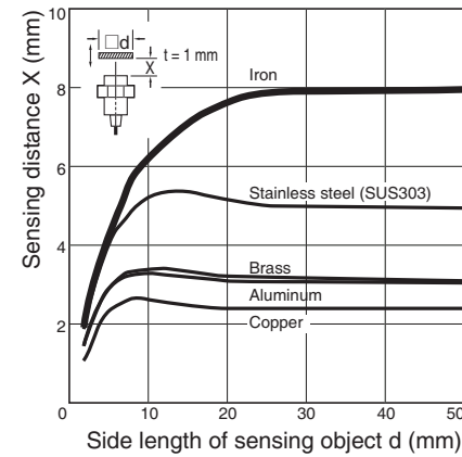
E2A-M12□N08/E2A-S12□N08
