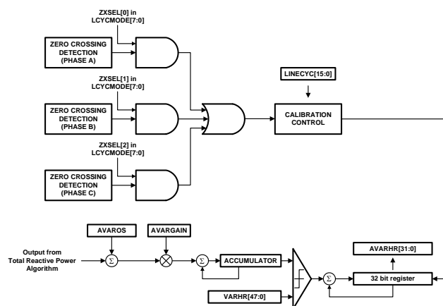
Figure 46. ADE7858 Line Cycle Reactive Energy Accumulation Mode
