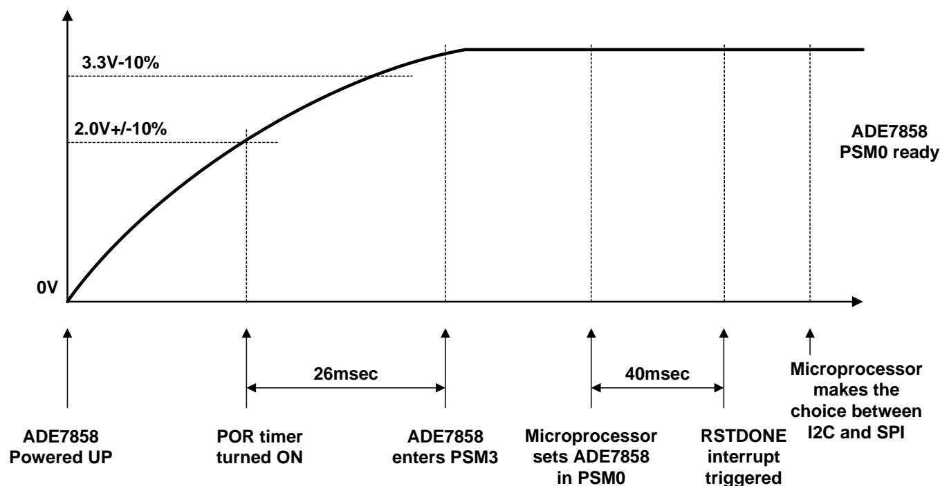
Figure 8. ADE7858 power up procedure
