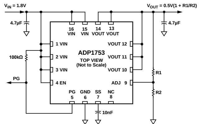
Figure 2. ADP1753 with Adjustable Output Voltage, 0.75 V to 3.3 V
