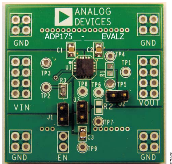
Figure 46. Evaluation Board
