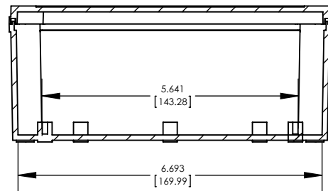
SECTION E-E
