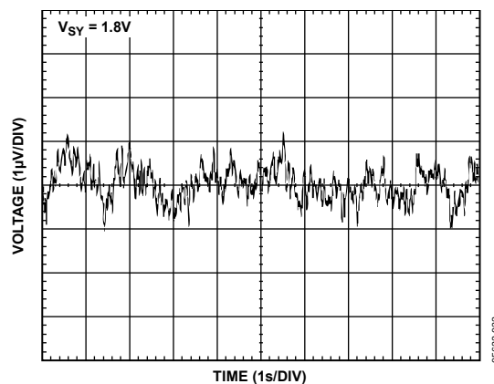
Figure 35. 0.1 Hz to 10 Hz Input Voltage Noise
