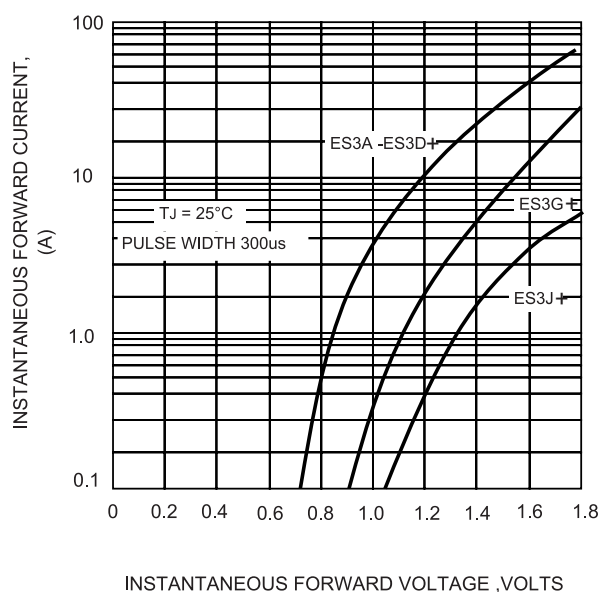
FIG.4-TYPICAL FORWARD CHARACTERISTICS
