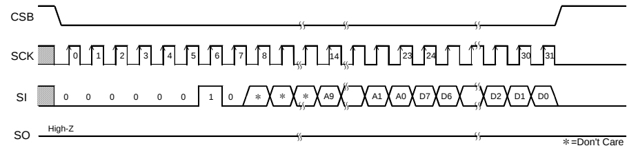
Figure 38. Write command
