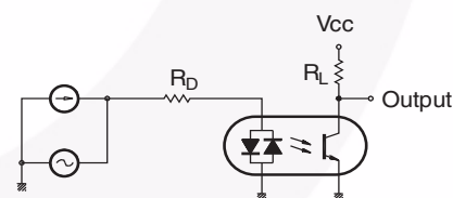
Fig. 19 Test Circuit for Frequency Response
