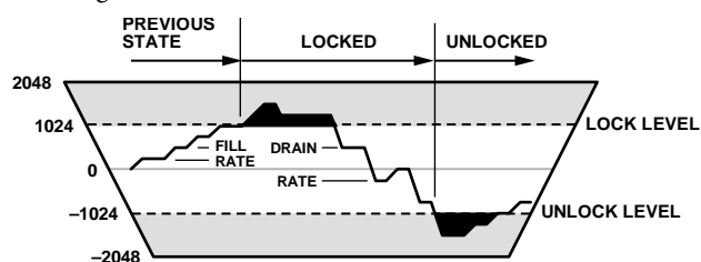
Figure 33. Lock Detector Diagram
