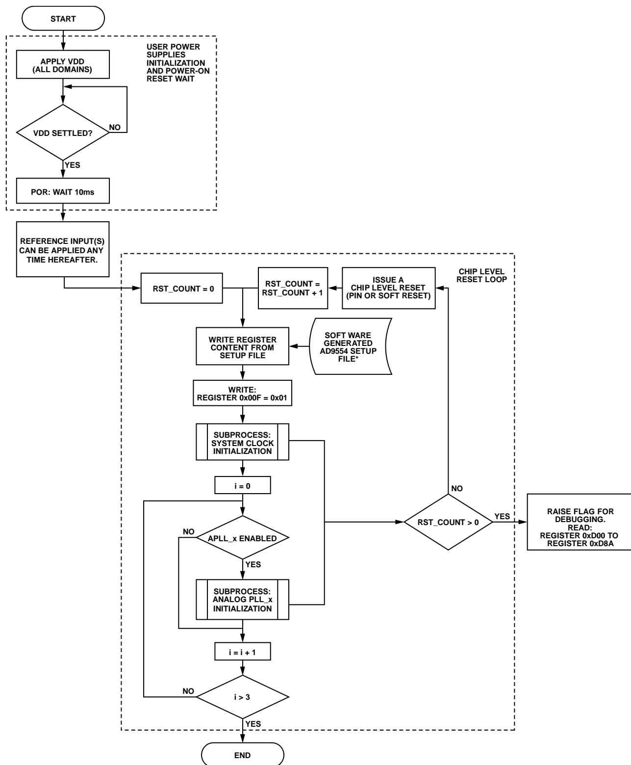
Figure 26. Main Process—Initialization
