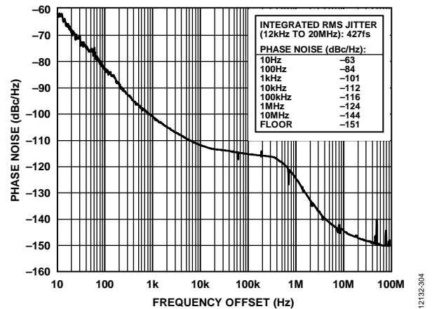
Figure 6. Absolute Phase Noise (Output Driver = 21 mA Mode), f_R = 19.44 MHz, f_{OUT} = 693.482991 MHz, DPLL Loop Bandwidth = 50 Hz, f_{SYS} = 49.152 MHz Crystal
