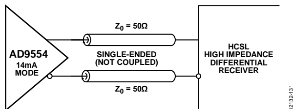
Figure 22. DC-Coupled HCSSL Receiver
