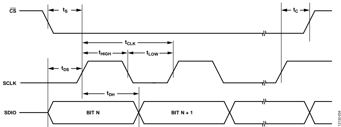
Figure 42. Serial Control Port Timing—Write
