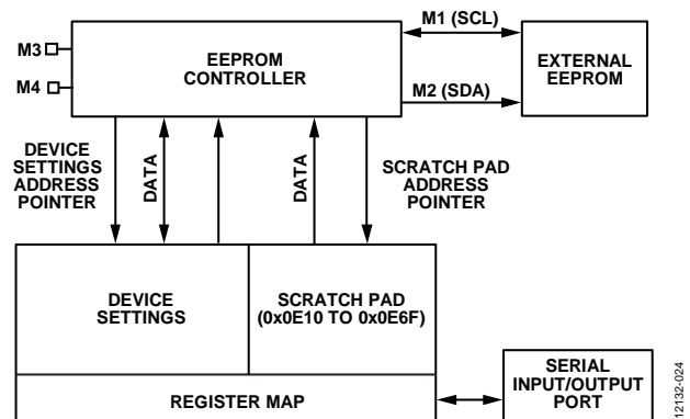
Figure 36. EEPROM Functional Diagram
