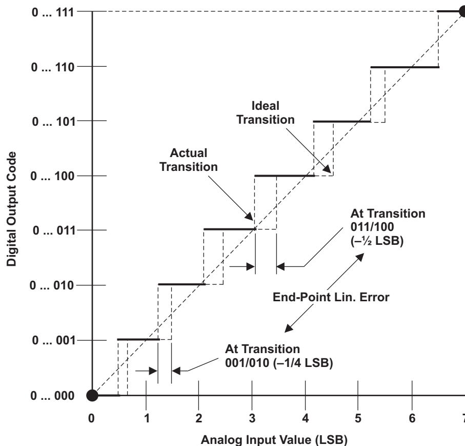
Figure 7-13. Integral Nonlinearity (INL) Error
