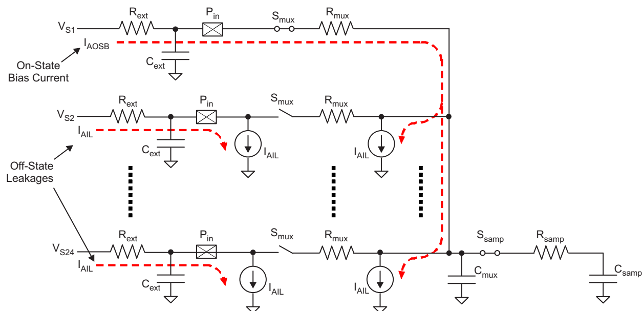
Figure 7-11. MibADC Input Equivalent Circuit
