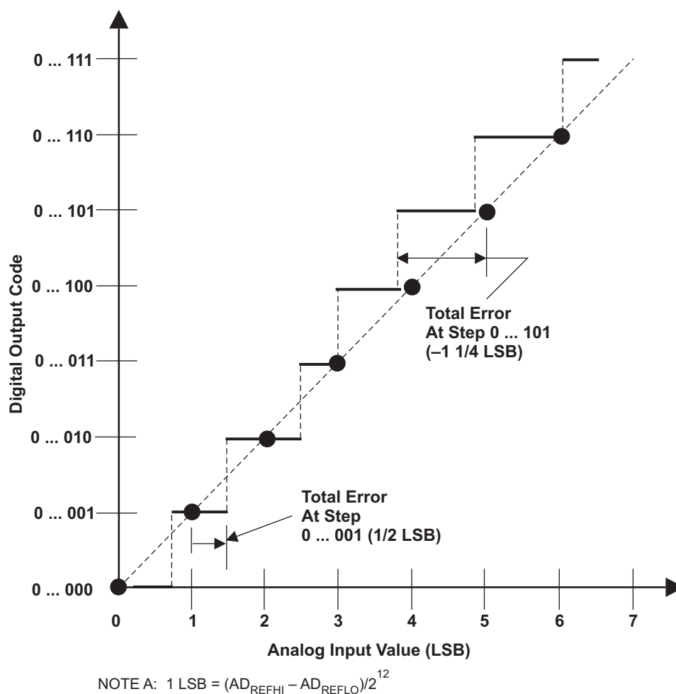
Figure 7-14. Absolute Accuracy (Total) Error
