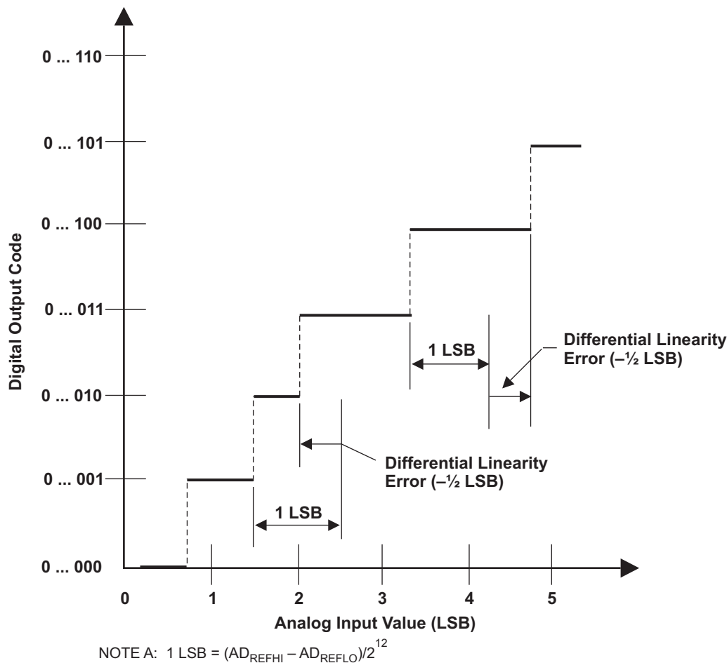
Figure 7-12. Differential Nonlinearity (DNL) Error
