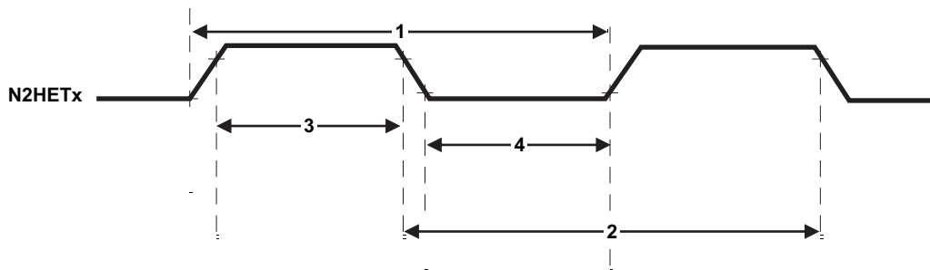
Figure 7-15. N2HET Input Capture Timings
