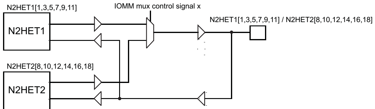
Figure 7-17. N2HET Monitoring
