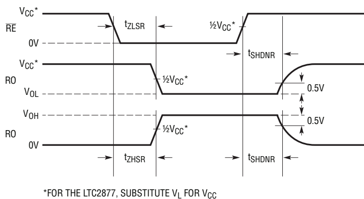
Figure 9. Receiver Shutdown Timing Measurements
