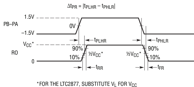
Figure 7. Receiver Propagation Delay Measurements
