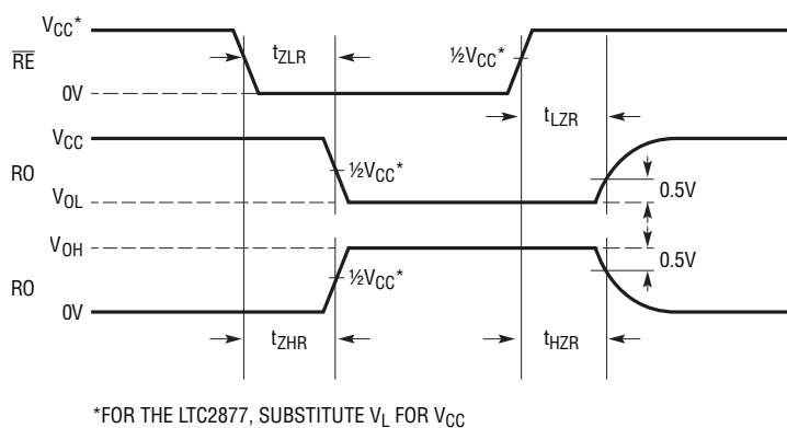
Figure 8. Receiver Enable and Disable Timing Measurements
