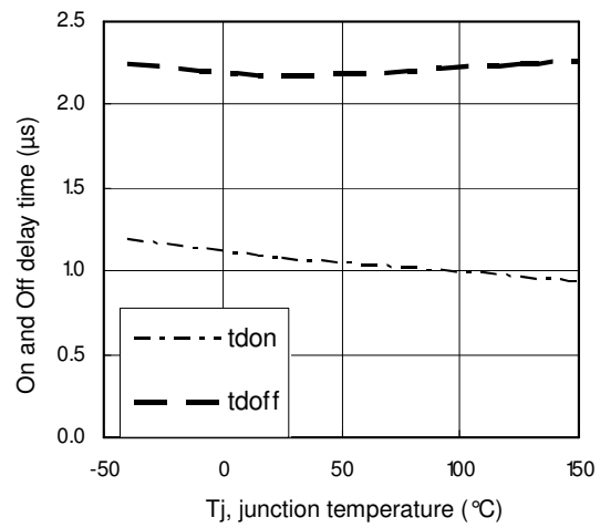
Figure 8 – tdon / tdoff (μs) Vs Tj (°C)
