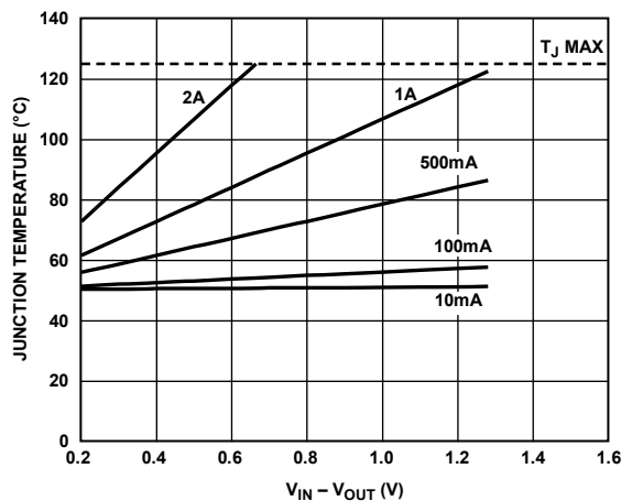
Figure 37. 6400 mm 2 of PCB Copper, T_A = 50^\circ\text{C}
