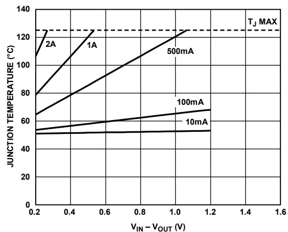
Figure 39. 25 mm 2 of PCB Copper, T_A = 50^\circ\text{C}
