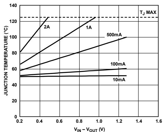
Figure 38. 500 mm 2 of PCB Copper, T_A = 50^\circ\text{C}
