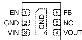
WDFN-6L 2x2
