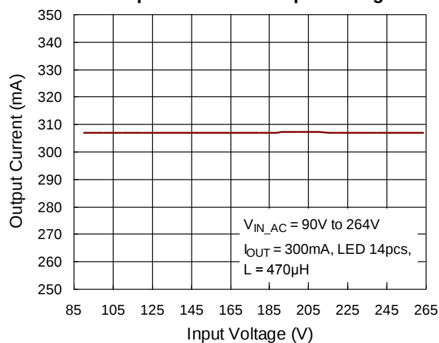
Output Current vs. Input Voltage
