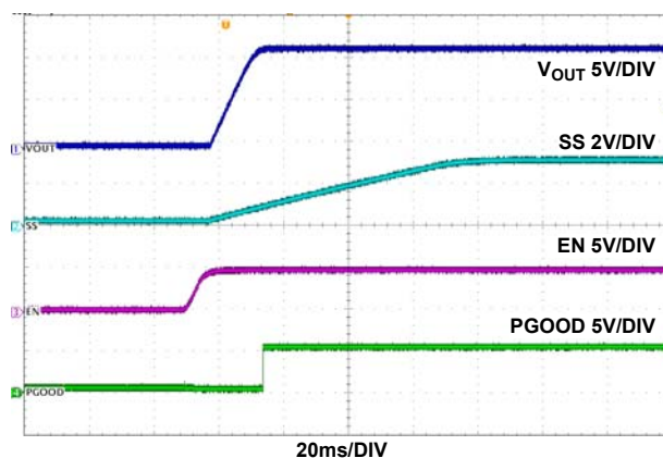
FIGURE 25. START-UP WAVEFORMS; MODE = DEM, LOAD = 0A, V_{IN} = 48V
