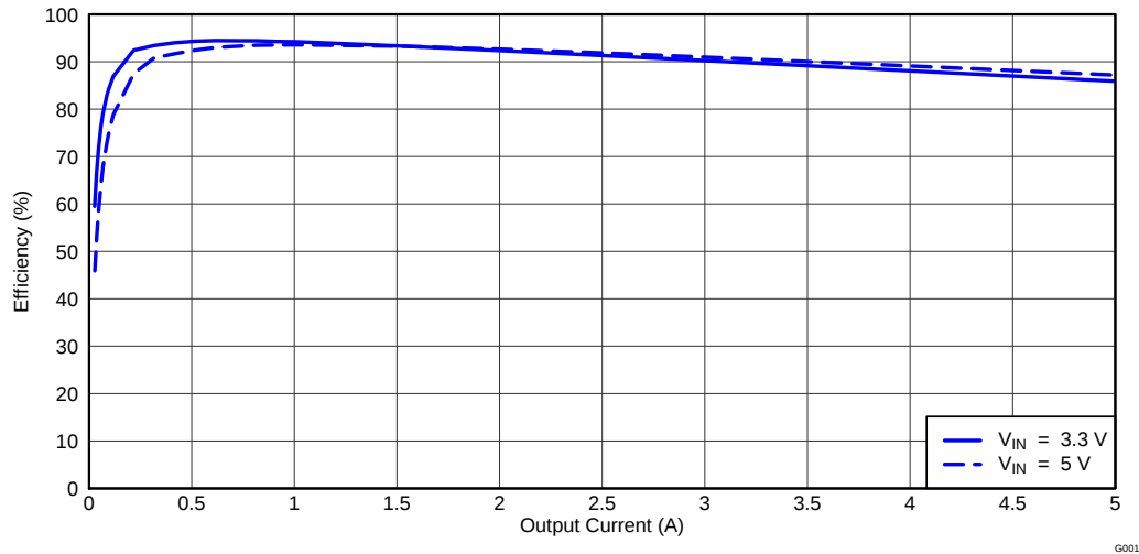
Figure 1. TPS54519EVM-037 Efficiency
